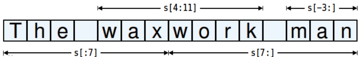
Figure 6 Sequence slicing
