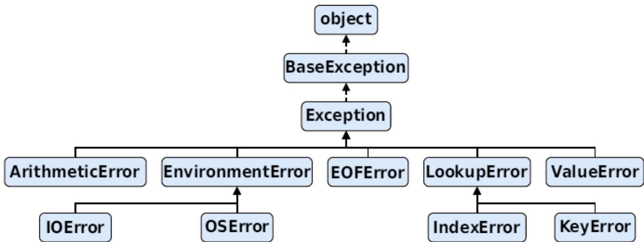
Figure 18: Some of Python's exception hierarchy
