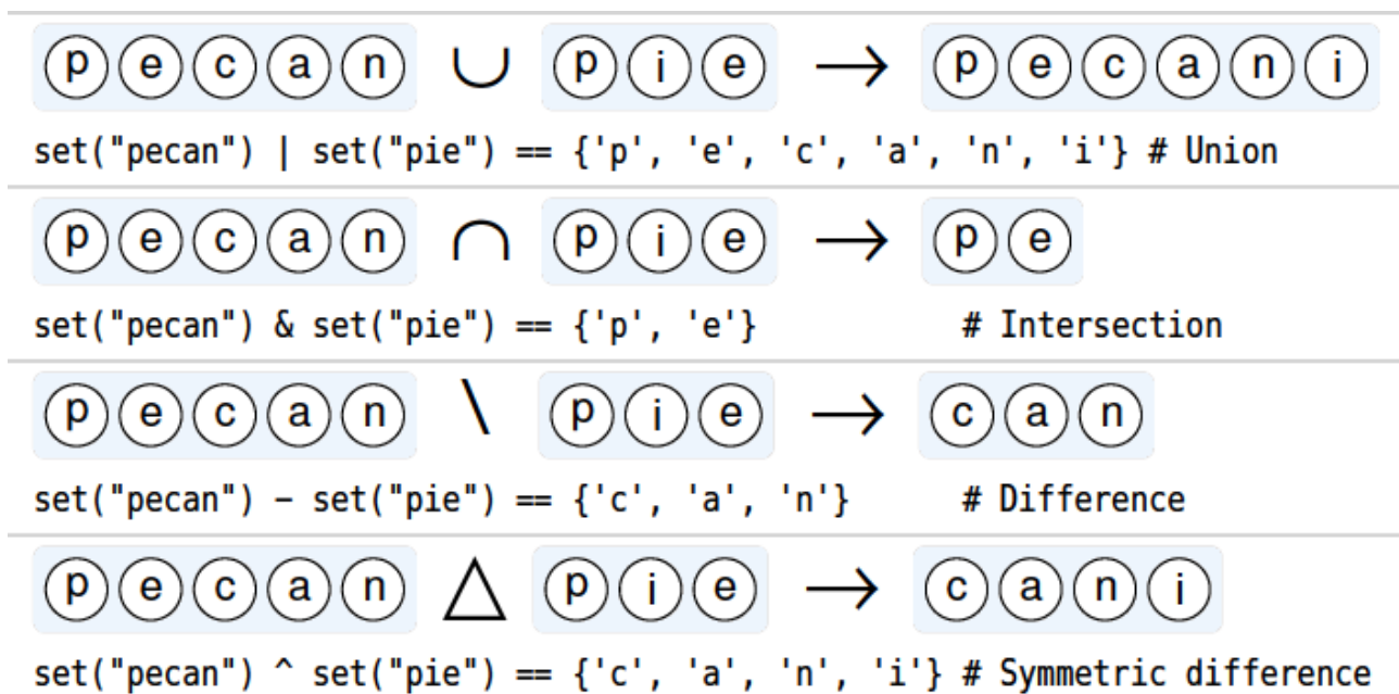
Figure 16: The standard set operators
