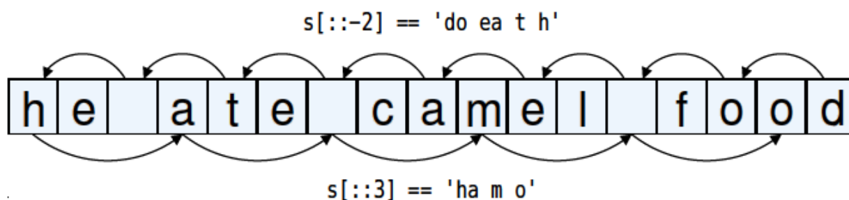
Figure 7 Sequence striding
