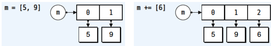
Figure 4: Augmented assignment of a mutable object
